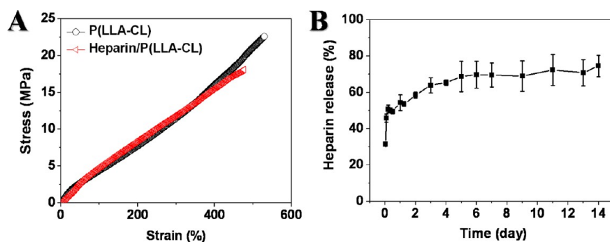
Figure 3. (A) Representative stress–strain curves of P(LLA-CL) and heparin-loaded P(LLA-CL) nanofiber grafts; (B) in vitro release of heparin from the heparin-loaded P(LLA-CL) nanofibers.
